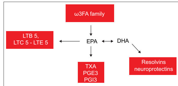
Figure 2 Synthesis of eicosanoids from \omega 3 FA: 3 series prostanoids TXA3, PGE3 and PGI3 and 5 series leukotrienes LTB5, LTC5-LTE5. Modified from Barbalho et al [33] and Din et al [37]
